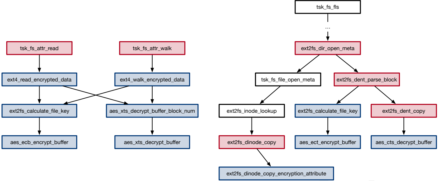
Figure 3: Overview of functions of The Sleuth Kit (TSK), including unmodified functions (white), new functions (blue), and modified functions by us (red).
