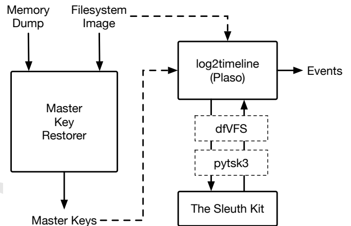
Figure 2: Overview of the modules and tools we extended or implemented and how they interact with each other.
